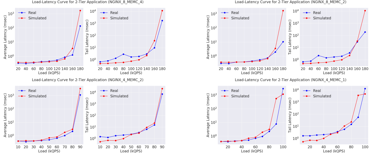
Figure 5: Validation of the two-tier (NGINX-memcached) application across different thread configurations for each microservice.
